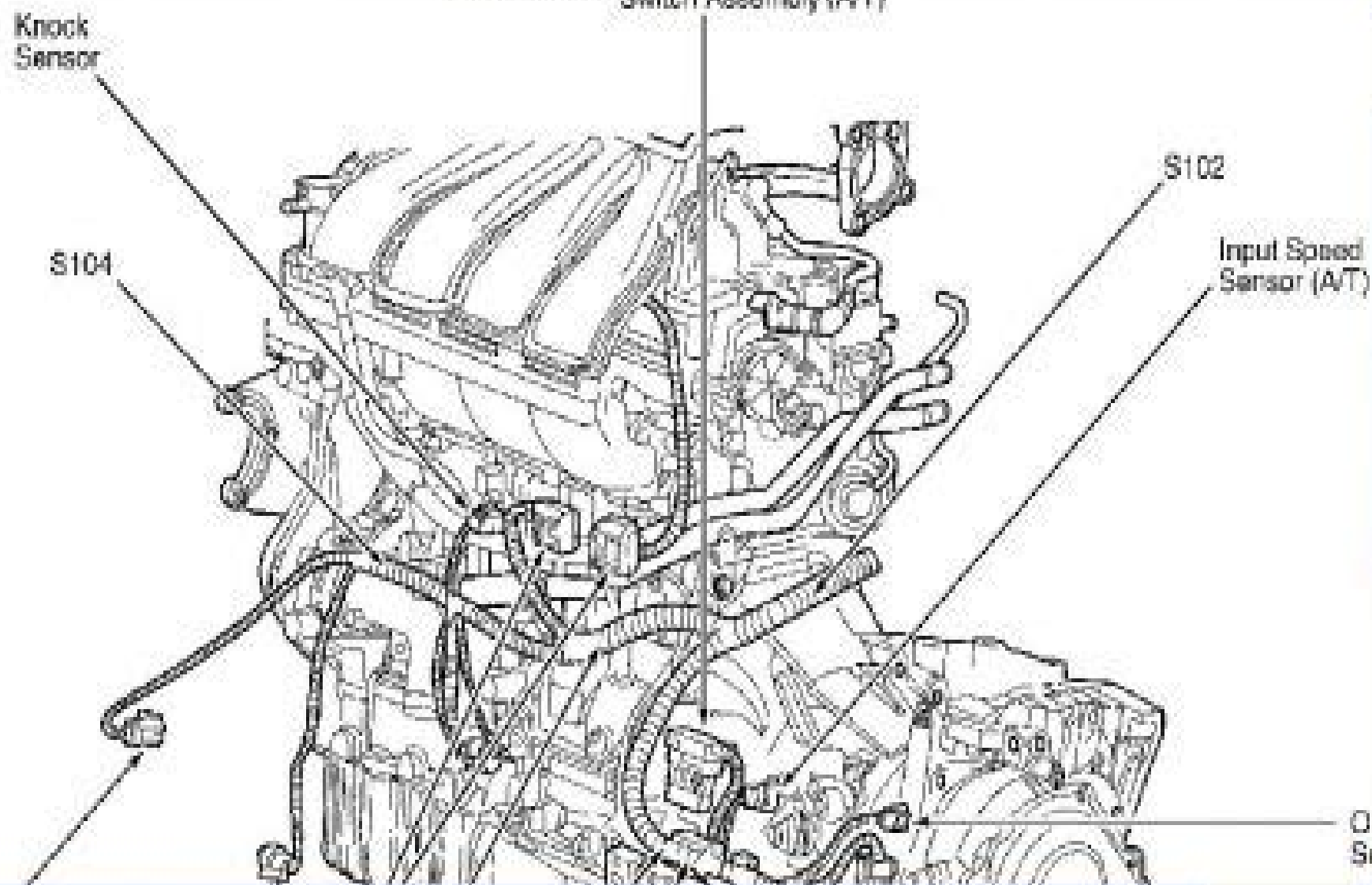
Fig. 2: Left Side Of Engine/Transaxle (2.4L Non-Turbo)
