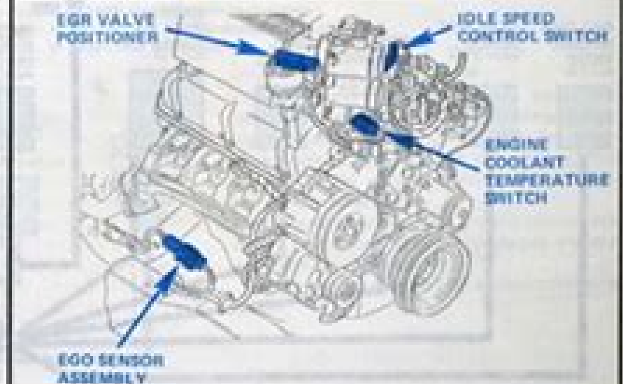
Figure 4 - RH Side of 5.0L EFI Engine
