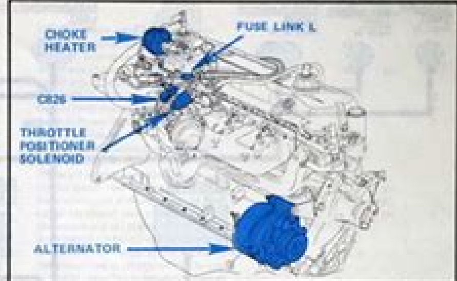
Figure 2 - RH Side of Heavy Duty 4.9L Engine
