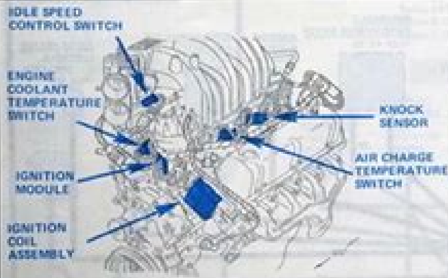
Figure 3 - LH Side of 5.0L EFI Engine
