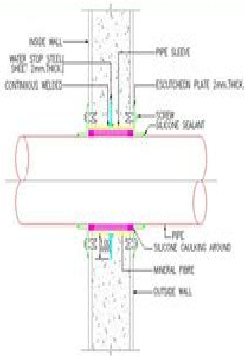
DETAIL OF PIPE SLEEVE THROUGH OUTSIDE WALL
