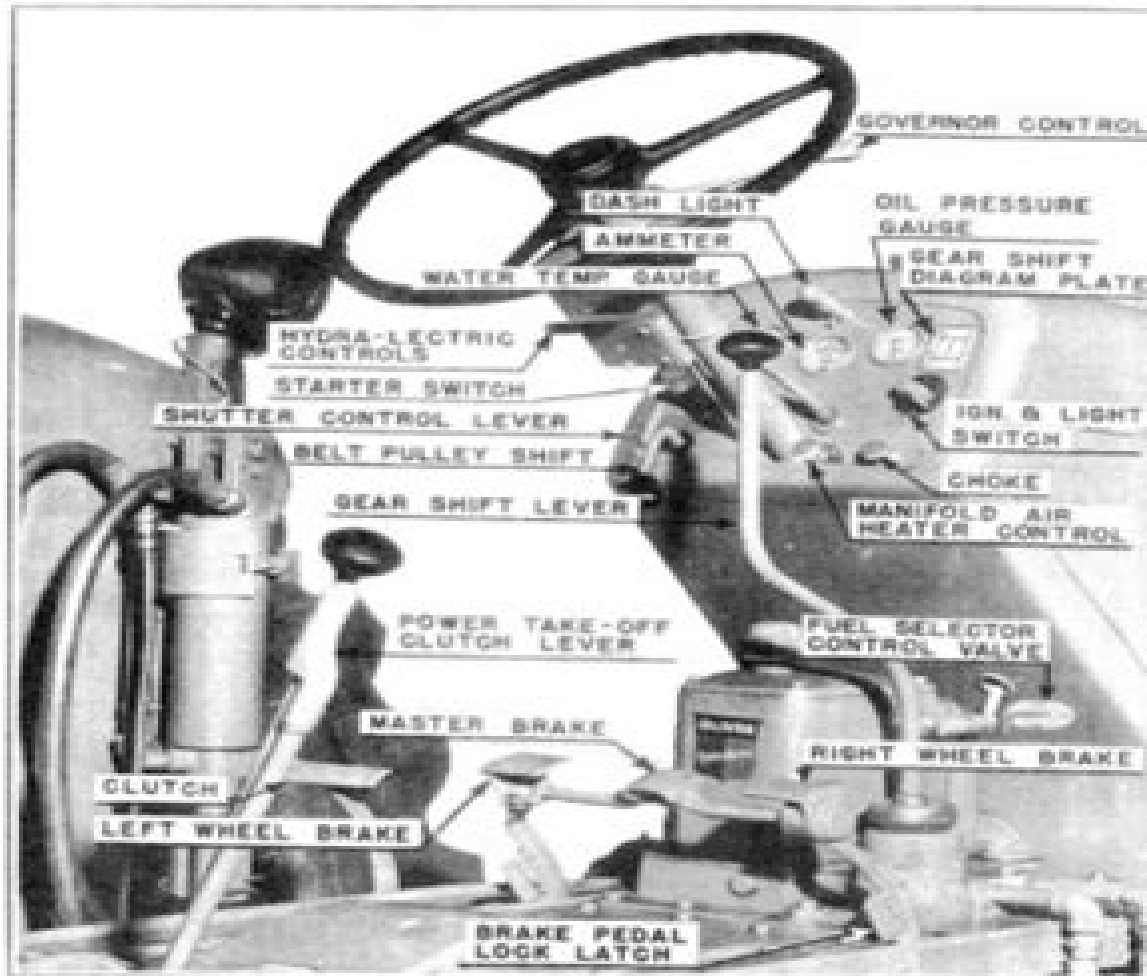
Figure 2 - MC and KD Controls
