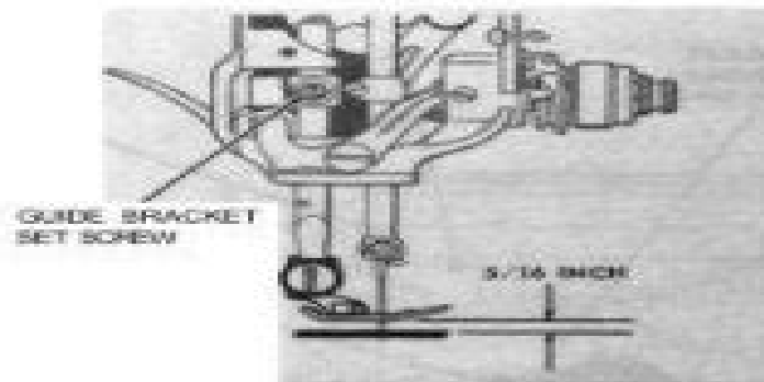
Fig. 8. Setting Presser Foot Height
