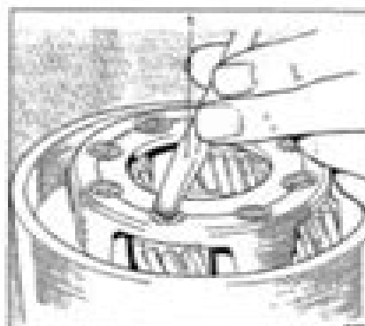
Fig. 11B-14 Staking a piston pin 1. Oil
