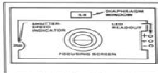
Figure 2 Viewfinder in Nikon FM
