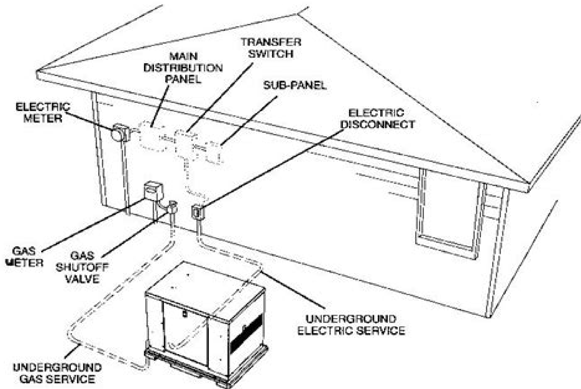
TYPICAL GENSET SITE
