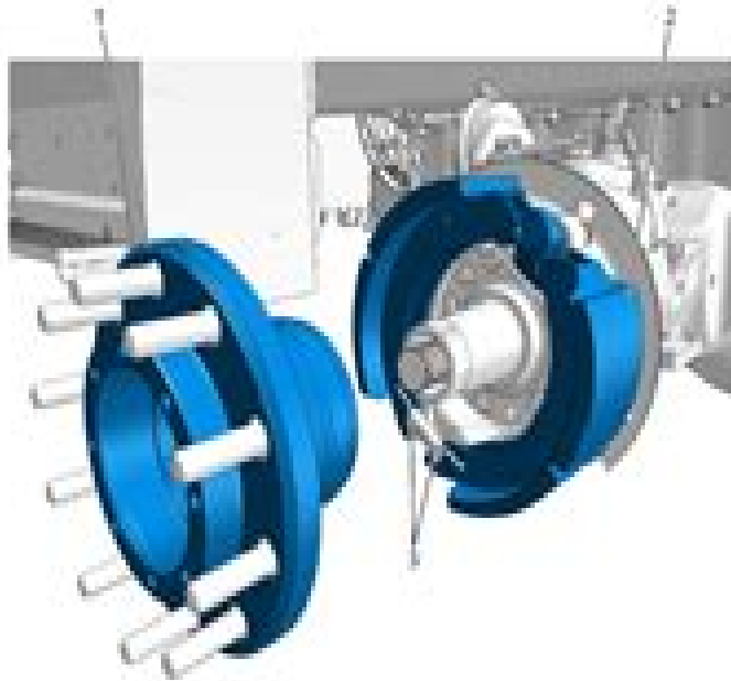
Figure 54 Wheel Hub and Brakes
