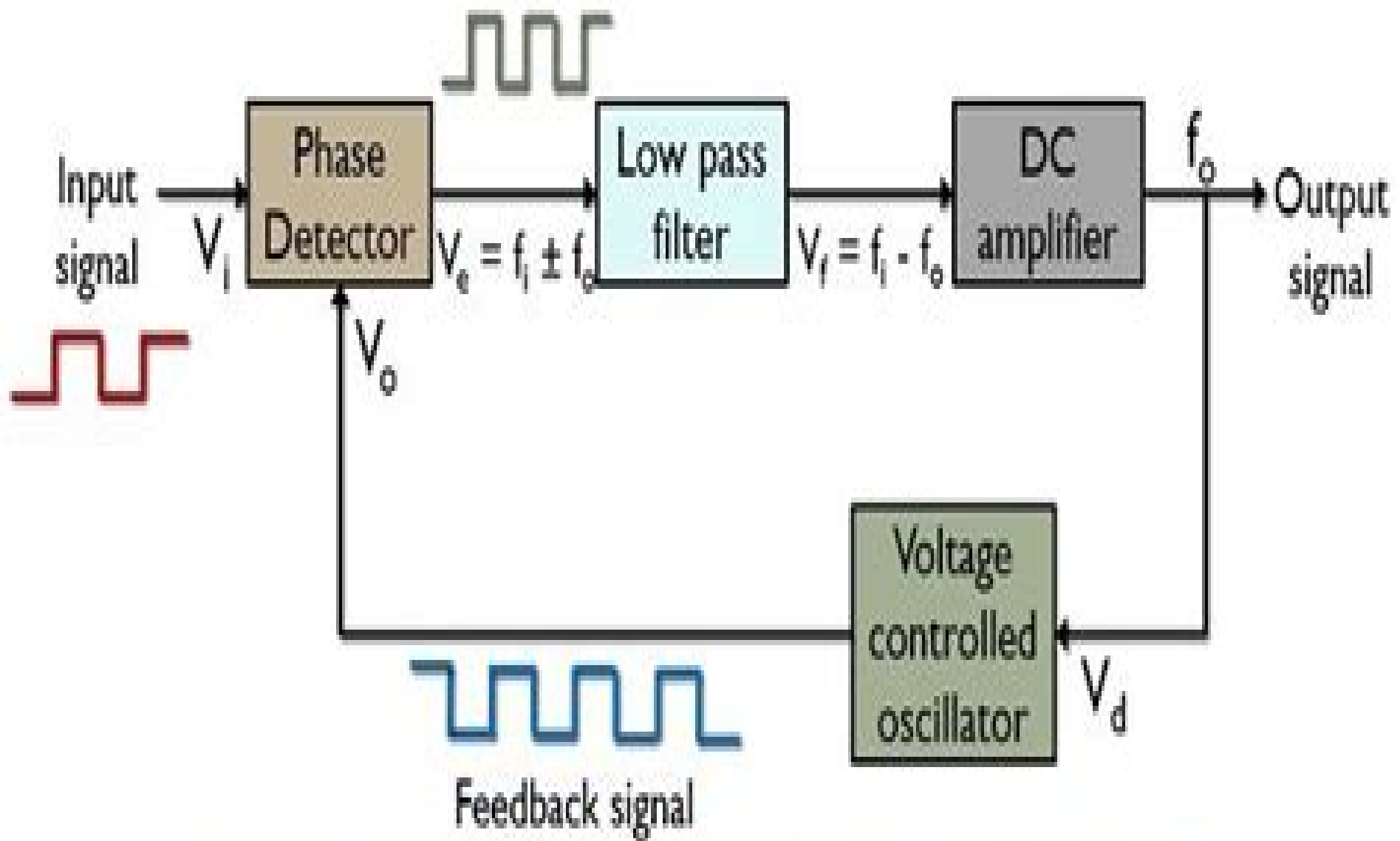
Block Diagram of Phase-Locked Loop
