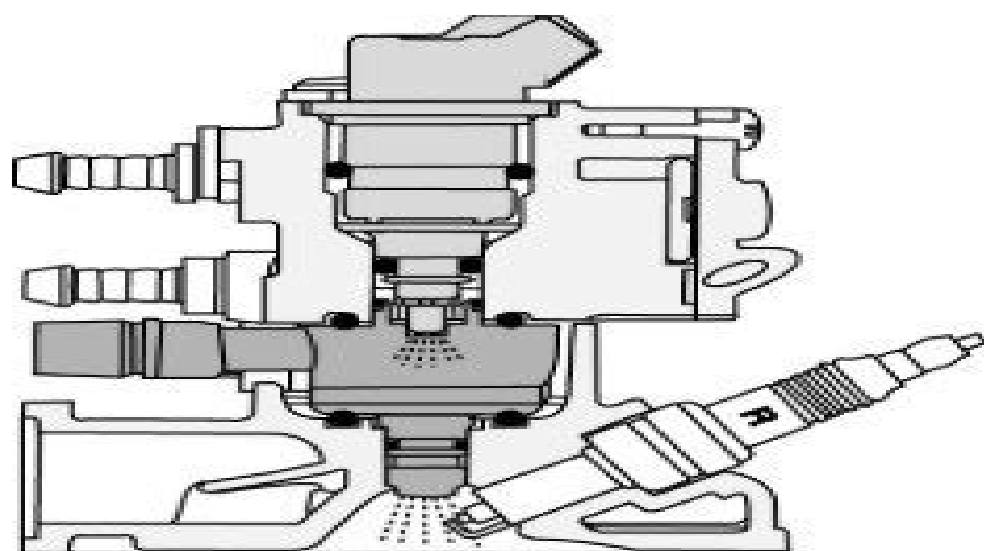
TSDI INJECTION SYSTEM FUNCTIONING PRINCIPLE (Two Stroke Direct Injection)
