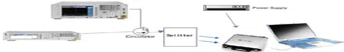
Figure-3. Configuration for Adjustment and Test of WIMAX mode
