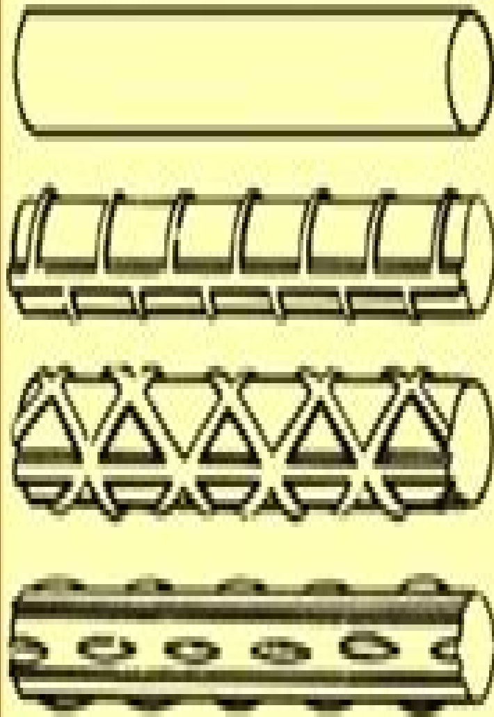
Plain, ribbed, or deformed bar
