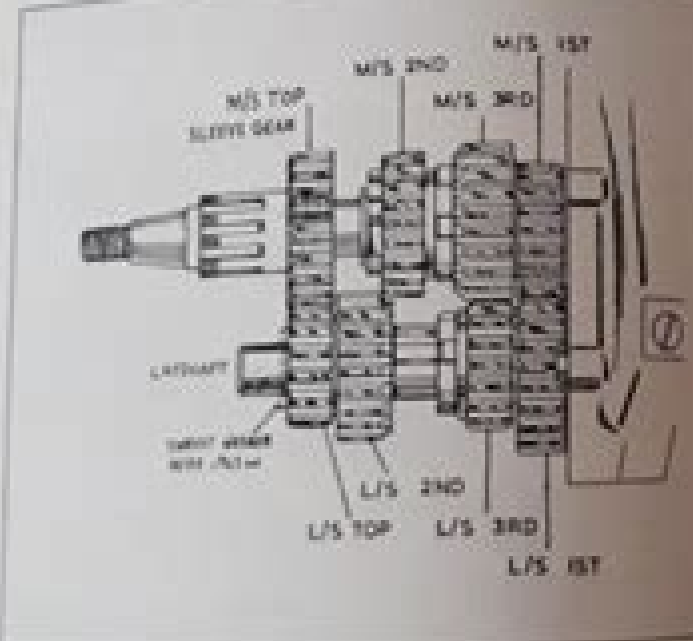
Illustration 9.15 - Gear cluster view from the rear
