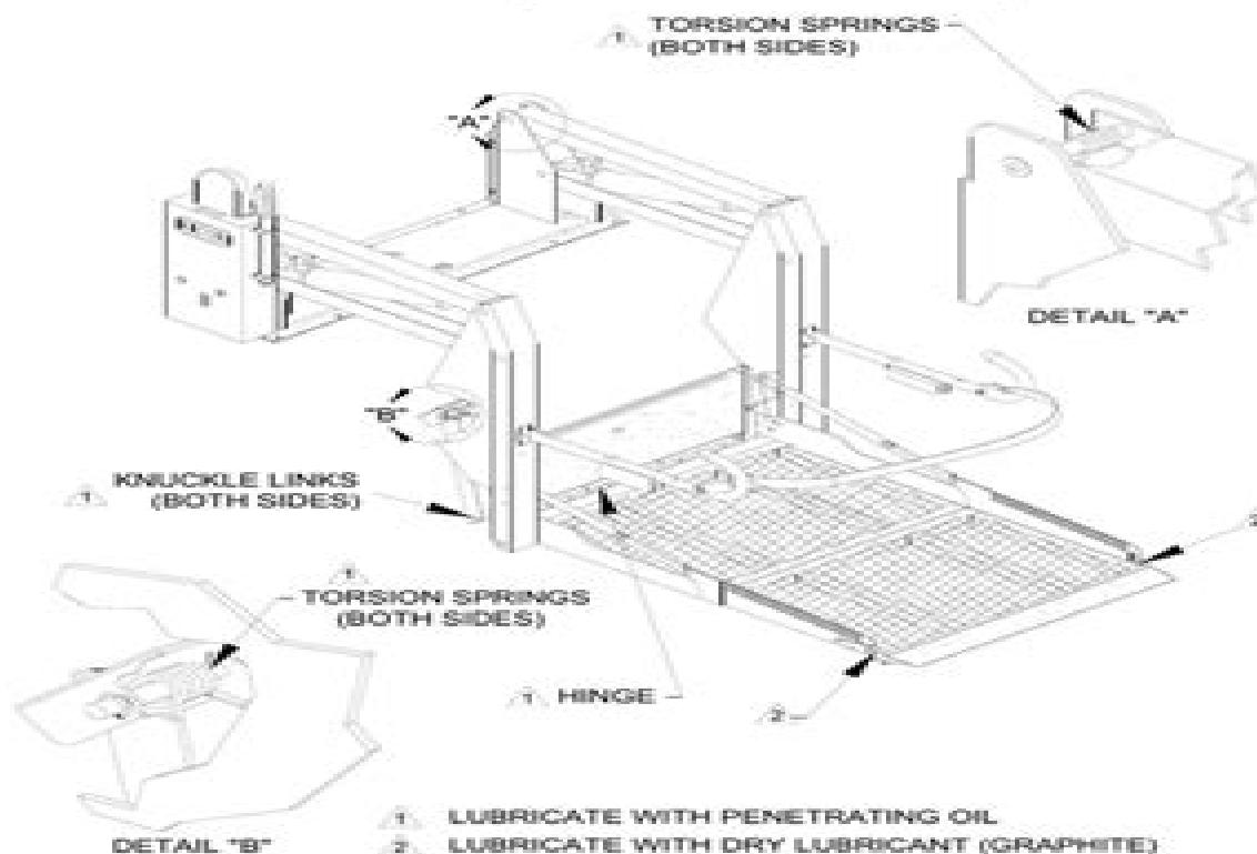
FIGURE 3-1: LIFT LUBRICATION POINTS
