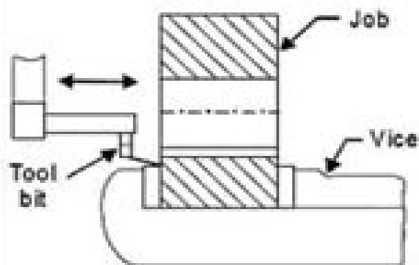
Keyway cutting
