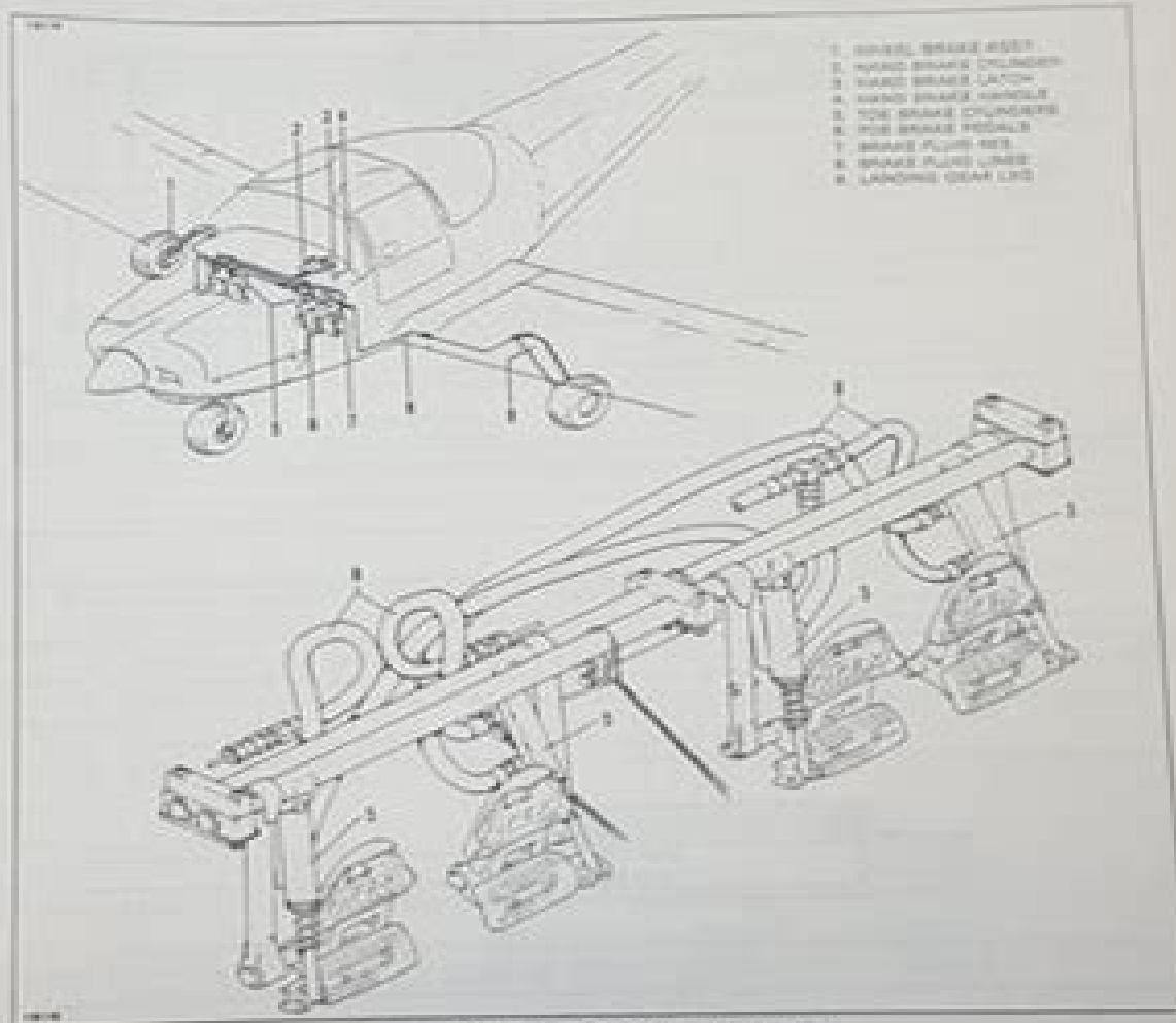
Figure 32-9. Toe Brake System Installation
