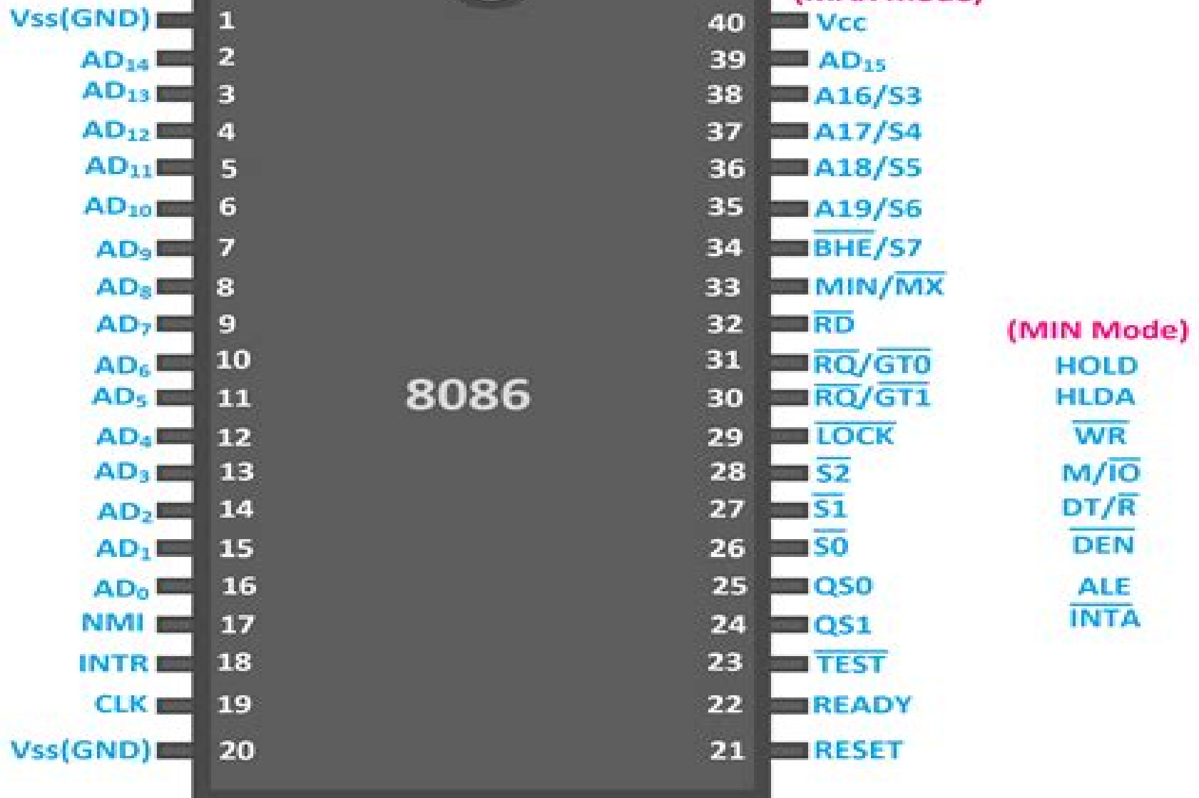
Microprocessor 8086 Pinout Diagram
