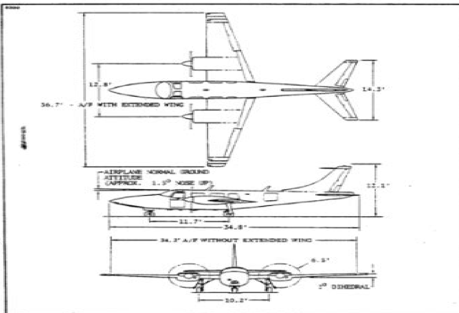
Figure 6-1. General Dimensions
