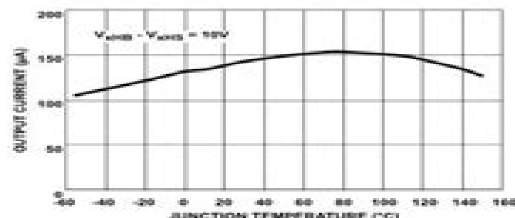
FIGURE 2. CHARGE PUMP OUTPUT CURRENT
