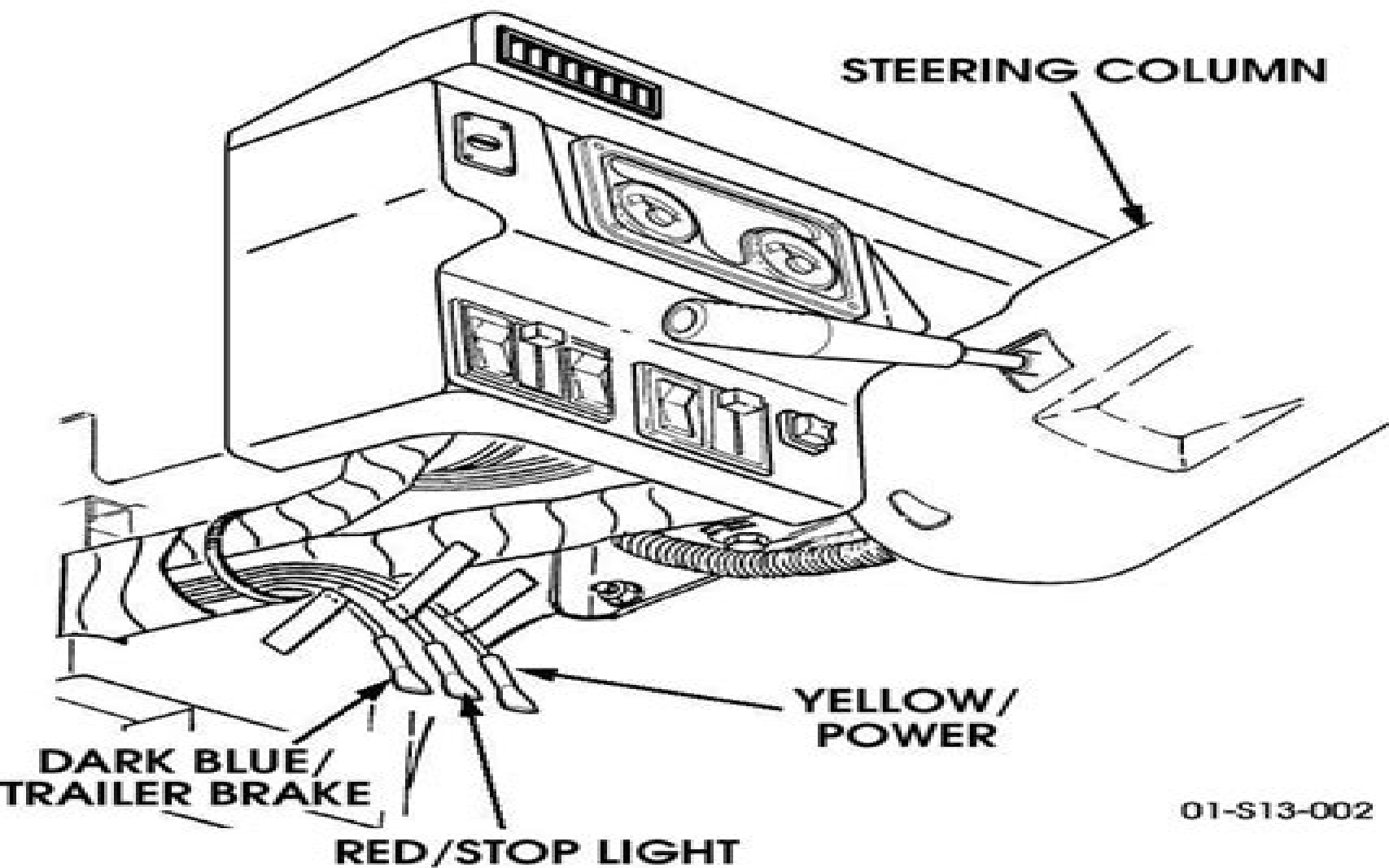
Figure 13-44: Trailer Brake Controller Wiring
