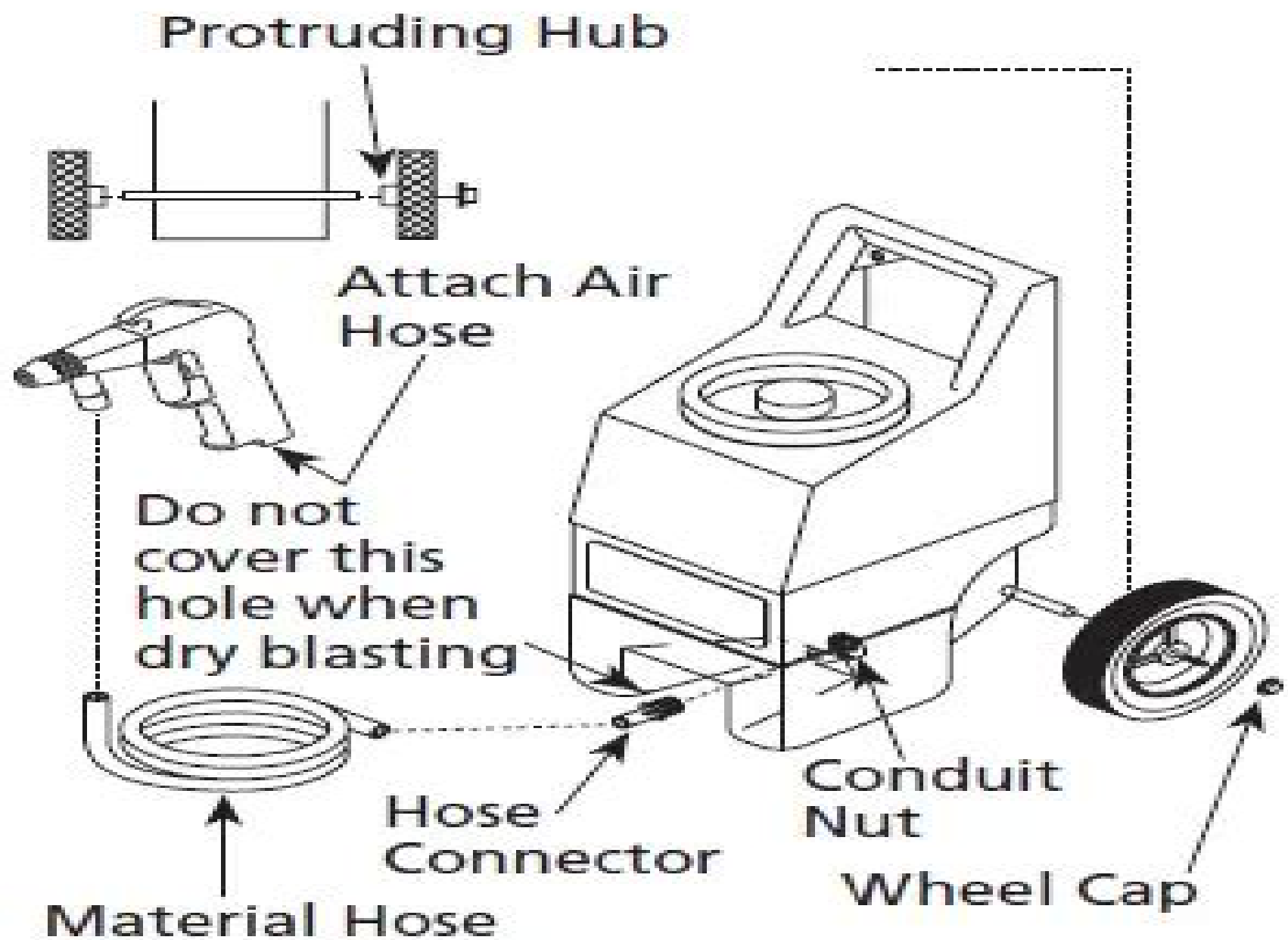
Figure 7 - Model AT121102
