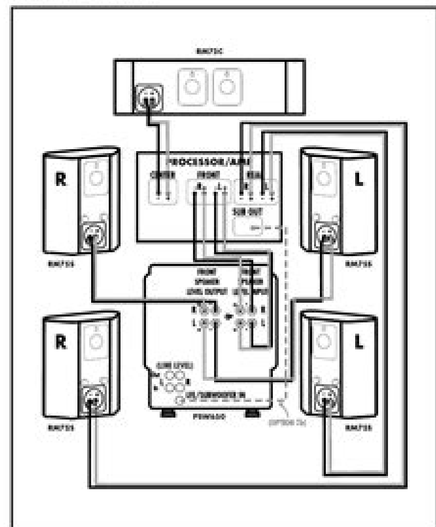
Figure 1: Dolby Digital 5 Speaker System, Page 4-1
