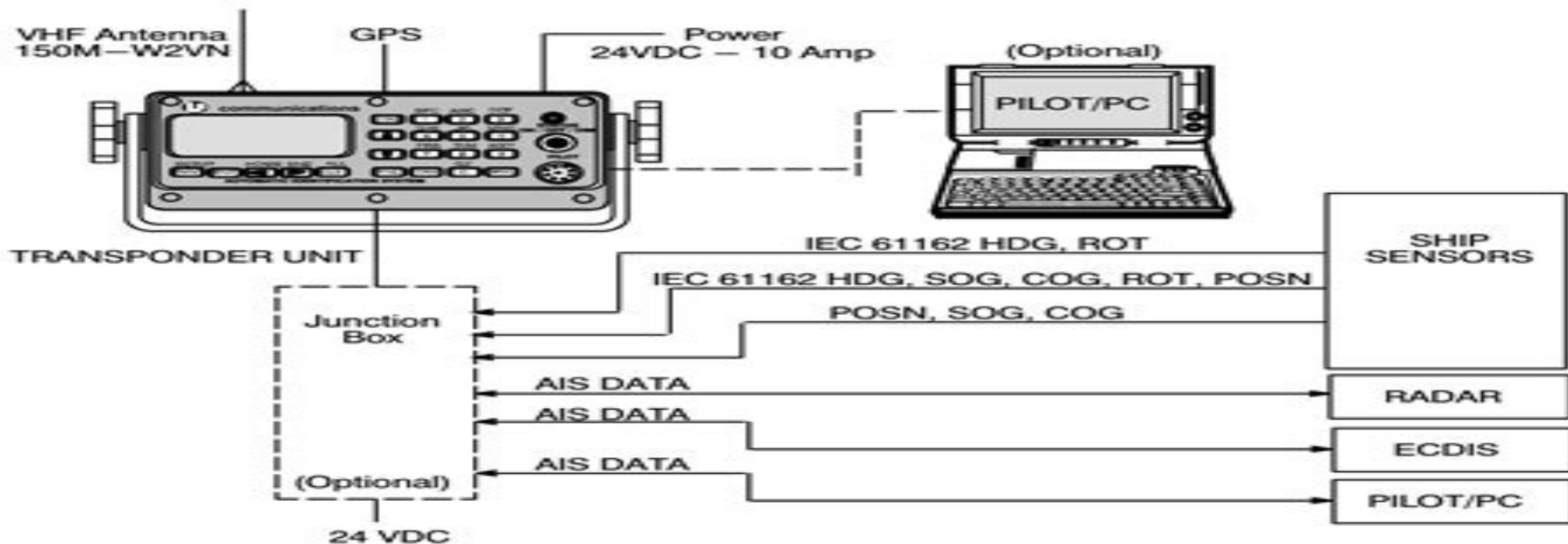
Figure 3-1. AIS Transponder Interconnection Diagram
