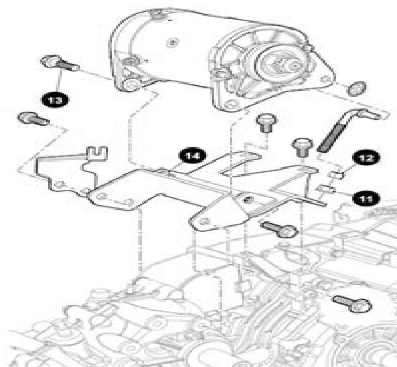
Figure 12 Starter/Generator
