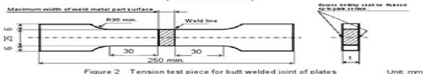
Figure 2 Tension test piece for butt welded joint of plates (No. 1 Test piece)
