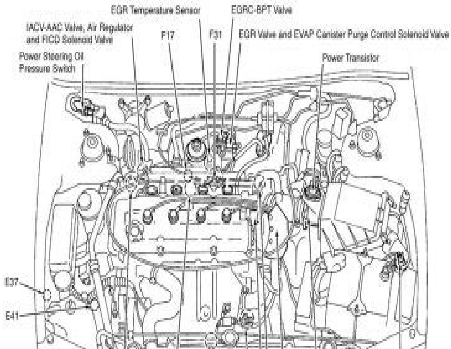
Fig. 1: Engine Compartment
