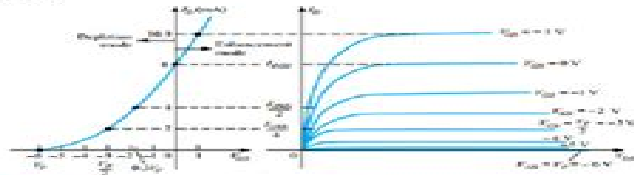
Figure 5.25 Static and transfer characteristics for an n-channel depletion-type MOSFET.
