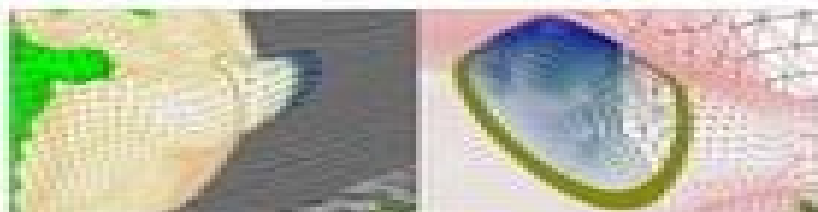
Advanced Mesh Editing tool allowing a modified or reconstructed well model bodies to greatly enhance productivity in depth imaging workflows
