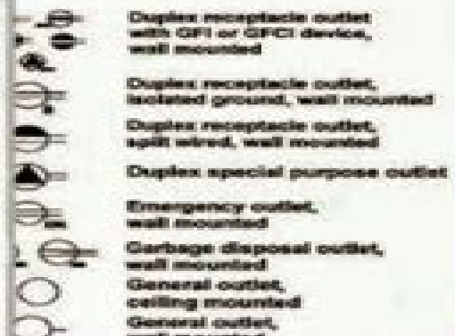
Outlet symbols
