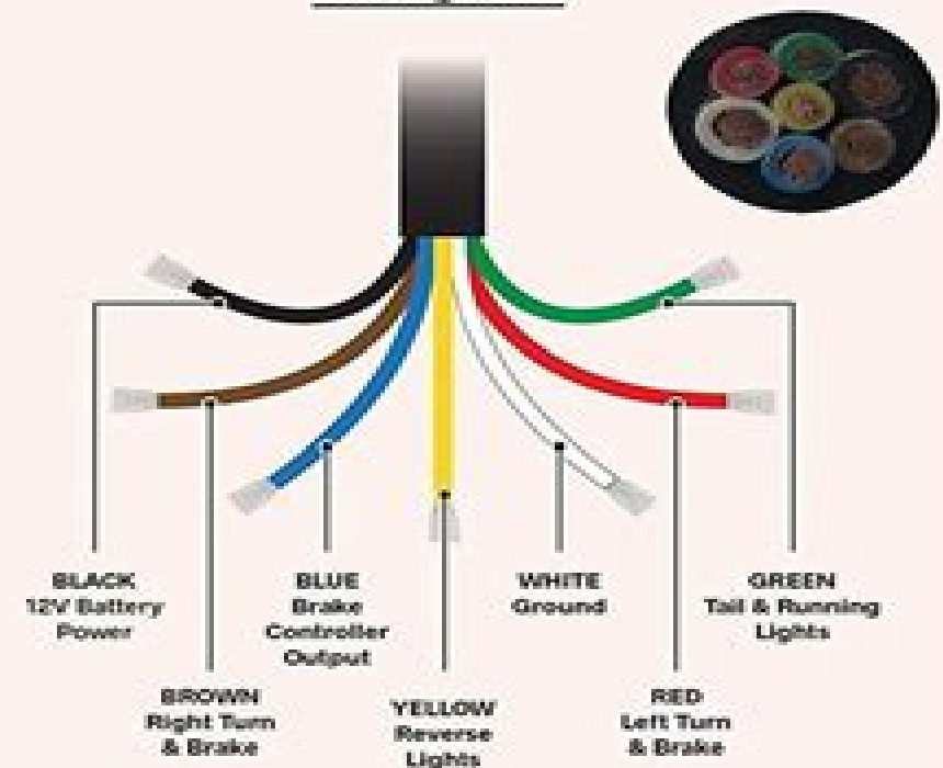
Wiring Side
