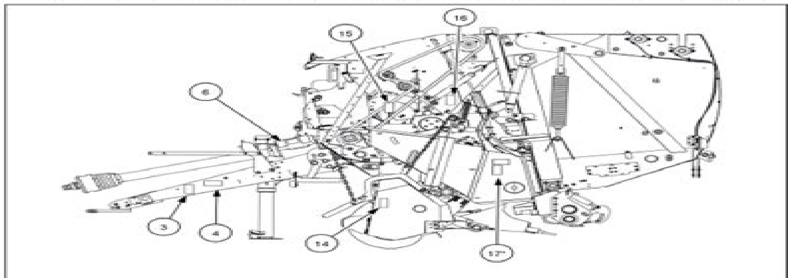
Left-hand view – CropCutter™ rotor cutter or SuperFeed™ rotor feeder baler – Without side shields
