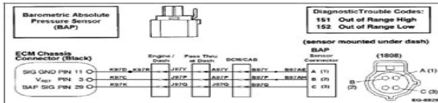
Figure 93 Barometric Absolute Pressure Sensor Circuit Diagram
