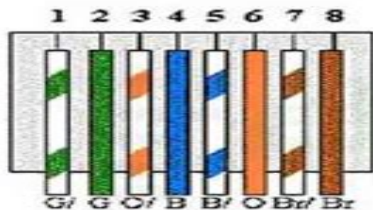
RJ-45 Male Plug
