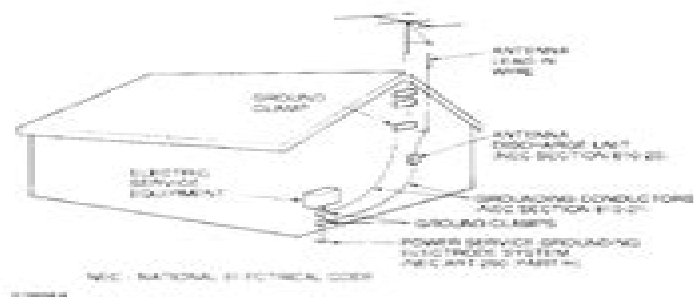
FIGURE 73.1: EXAMPLE OF ANTENNA GROUNDING AS PER NATIONAL ELECTRICAL CODE
