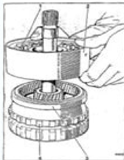
Fig. T13-3 Removing the reaction center assembly
