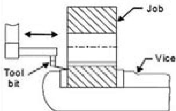
Keyway cutting
