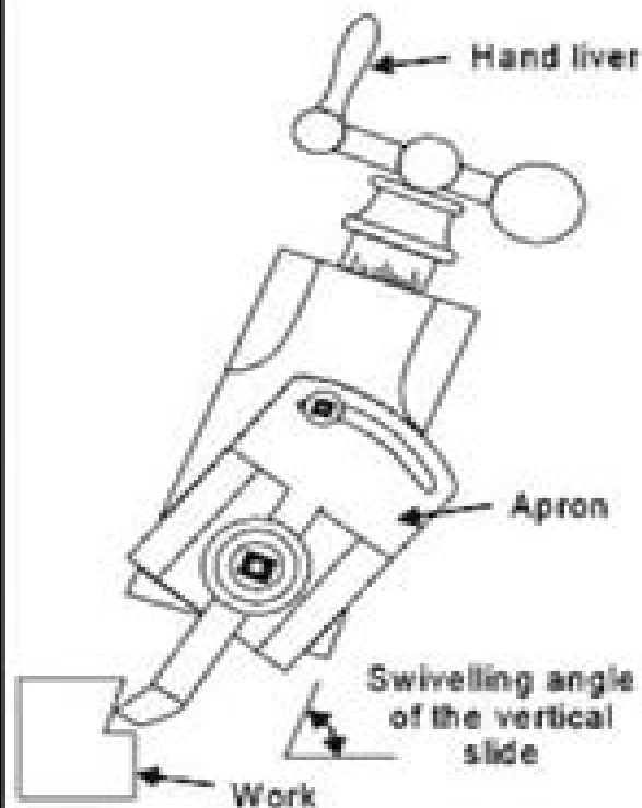
Machining inclined surface
