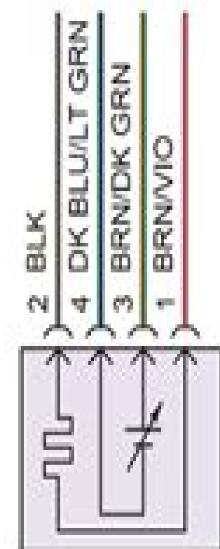
OXYGEN SENSOR 2/1
