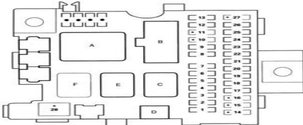
Fuses Under-dash Fuse/Relay Box (cont'd)
