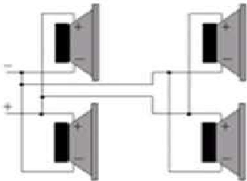
Wiring Four Speakers in Parallel
