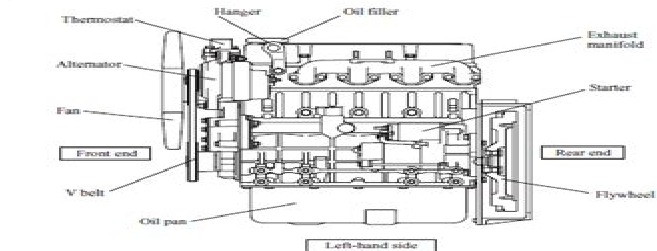
Engine LH side view
