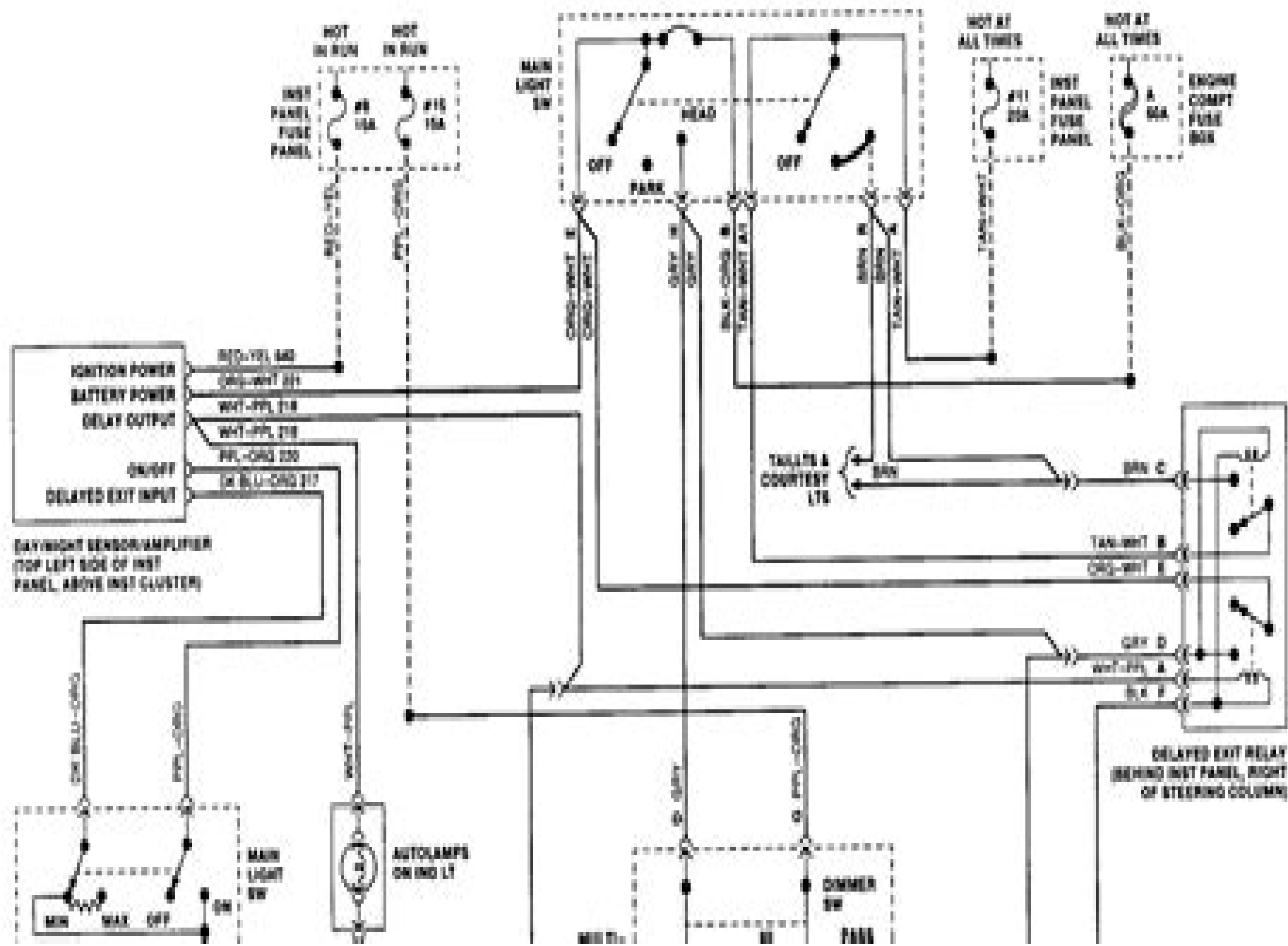
Fig. 6: Auto Headlight Dimmers Wiring Diagram Town Car (Automatic)
