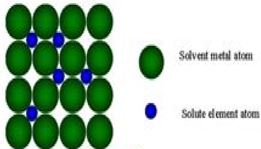
Interstitial solid solution
