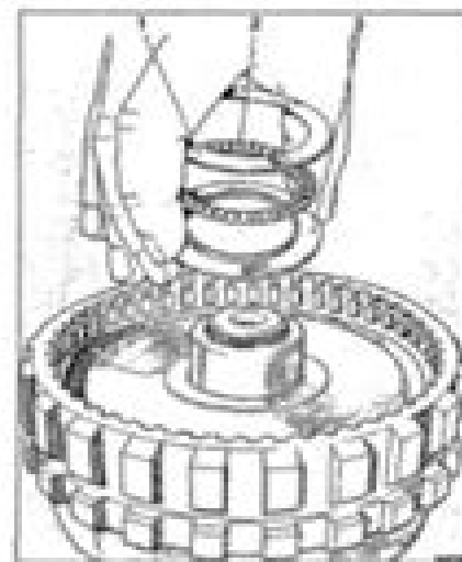
Fig. 715-16 Fitting the rear and thrust bearing to the outer face of the rear internal gear
