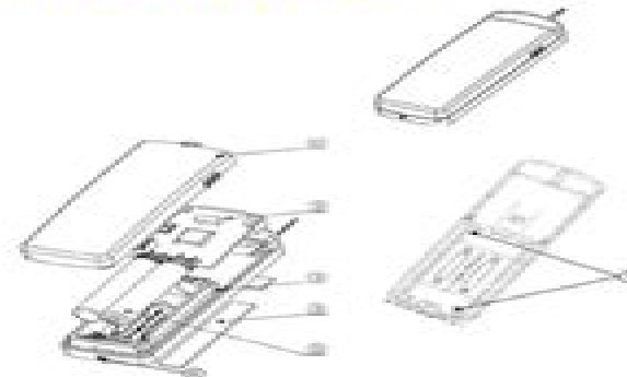
Figure 3 Mechanical Drawing
