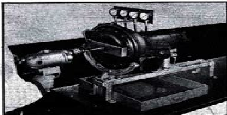
Fig. 125—Revolving Primary Pump
