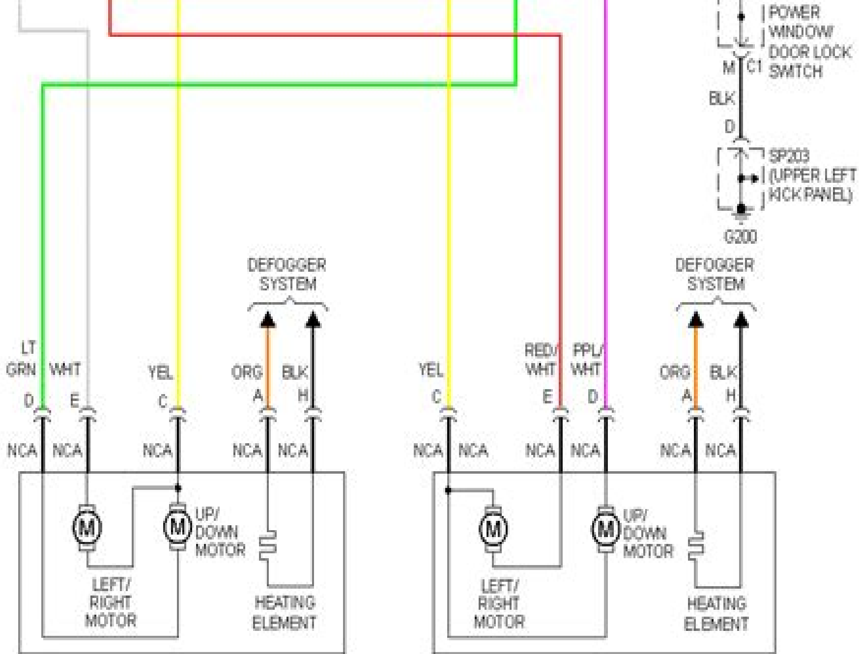
DRIVER OUTSIDE REARVIEW MIRROR
