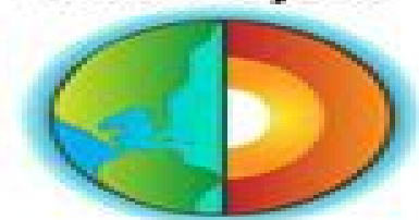
Earth Layers
