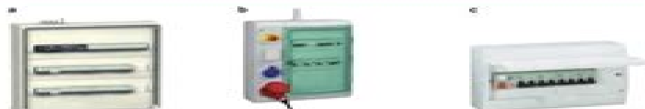
Fig. E29: Final distribution switchboards (a) Prisma Plus G Pack; (b) Kaepra; (c) mini-Pragma.
