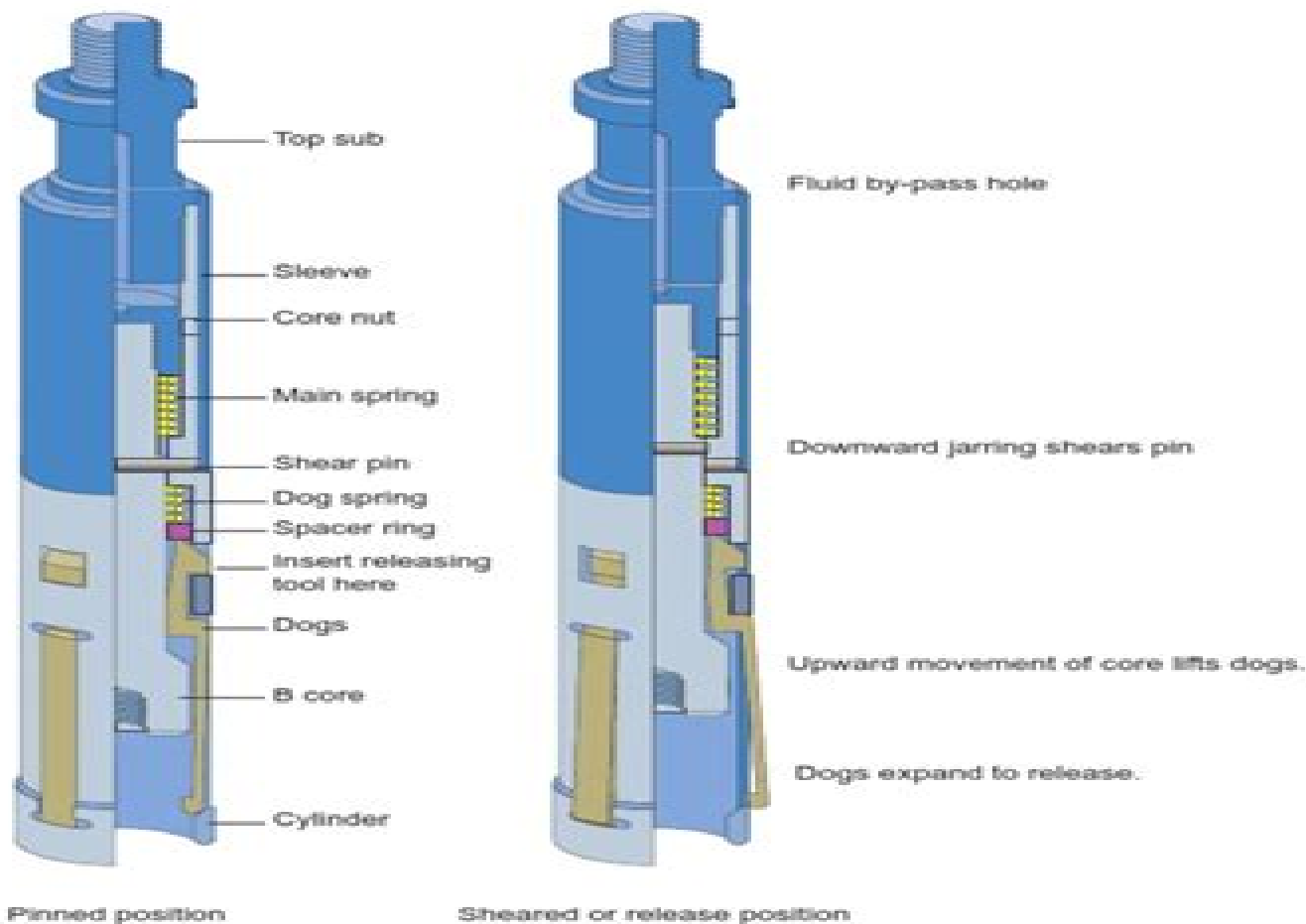
Figure 5-12: SB Pulling Tool
